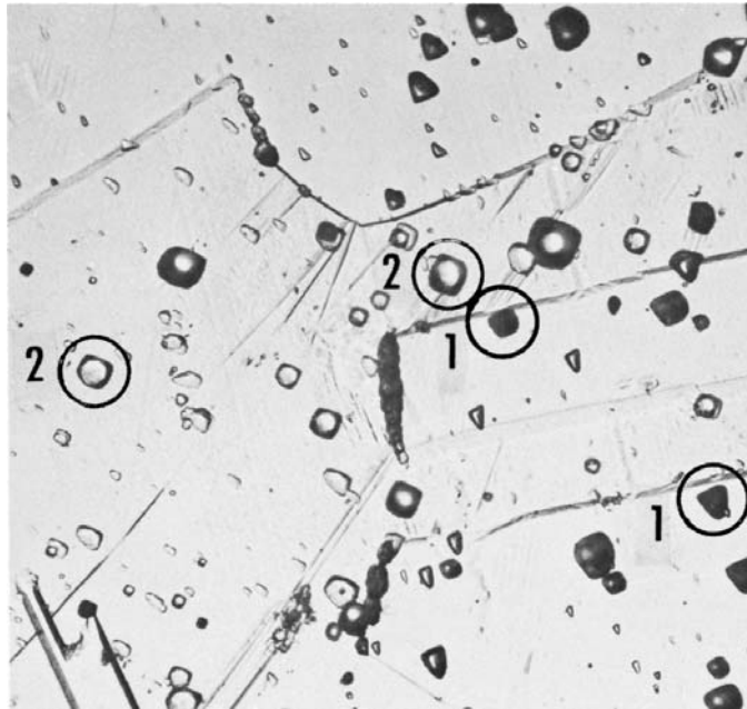
NOTE 1—To differentiate between the types of pits, use a magnification of 500× and focus in the plane of etched surface. The pits which now appear completely black are end grain pits.
