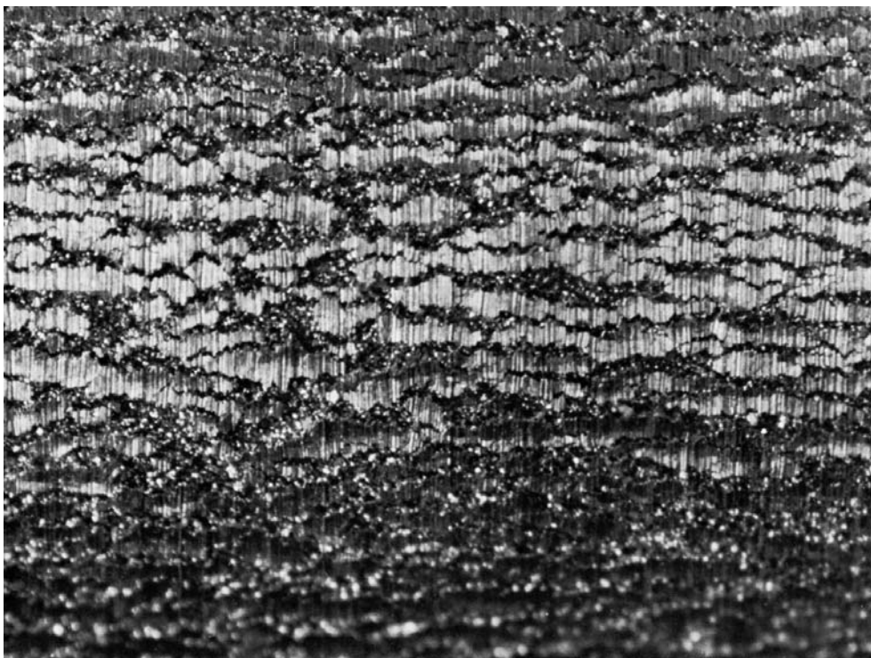
FIG. 12 Failing Test Specimen (Note the many intergranular fissures. Bent Area at 20 \times Magnification Before Reproduction.)
