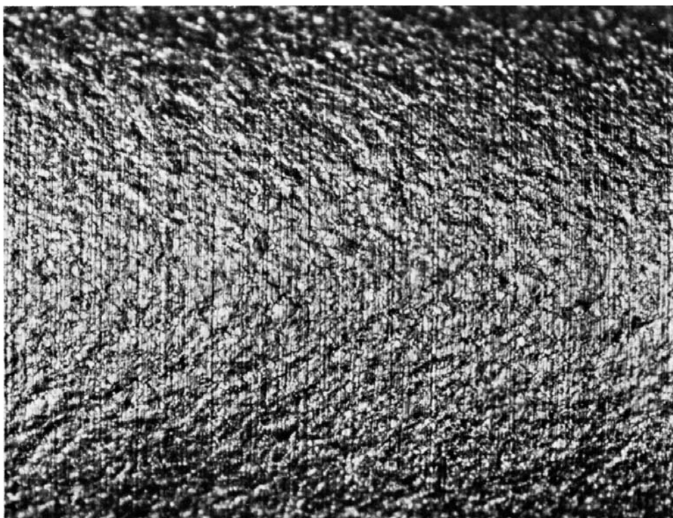
FIG. 13 Note the Traces of Intergranular Fissures and “Orange-Peel” Surface. Bent Area at 20x Magnification Before Reproduction.)
