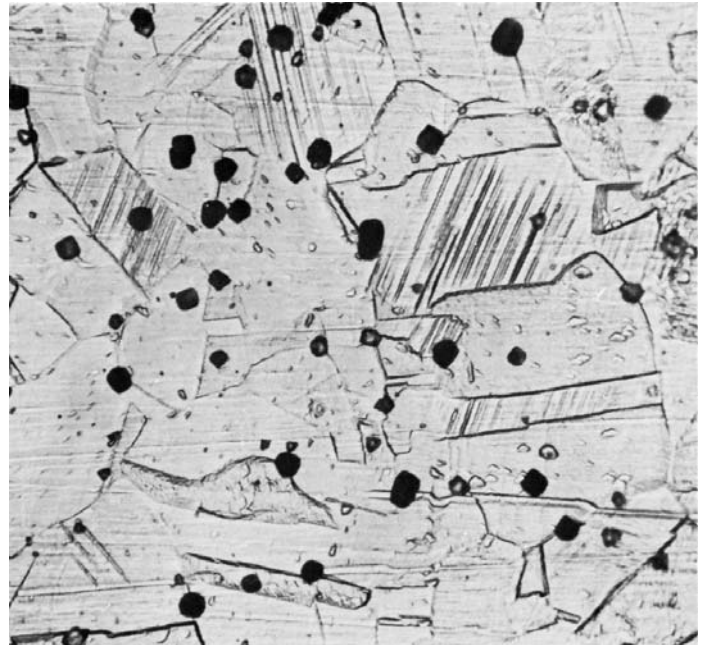
NOTE 1—This or a greater concentration of end grain pits at 500× (using standard etching conditions) indicates that the specimen must be tested when screening is for nitric acid test.
